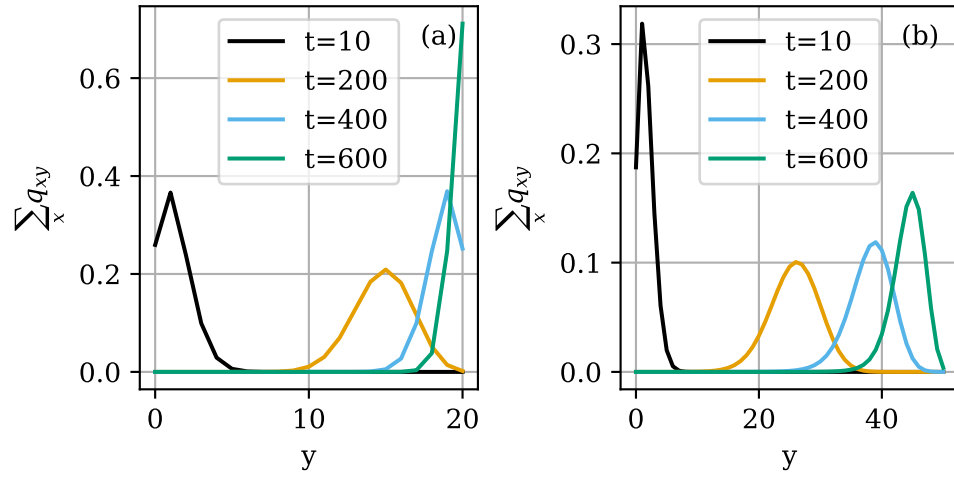
Figure 8: Evolution of N_w distribution for a pasture of size A = , for (a) N = and (b) N = .
