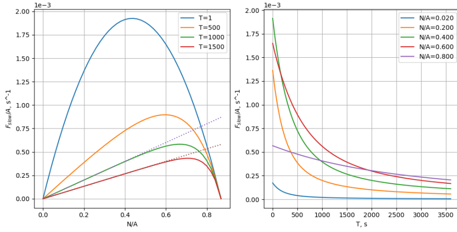
Figure 3: Plots of \frac{F_{slow}}{A} as a function of N and T .
