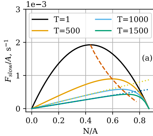
Figure 2. (a) Contours of F_{slow} as a function of N at constant T , (b) optimal sheep population and maximum wool production as a function of T , normalized to pasture size. The dashed line traces the optimal N and F_{slow} as T increases.
