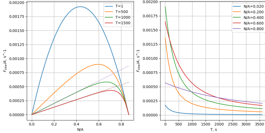
Figure 1: Plots of \frac{F_{slow}}{A} as a function of N and T .
