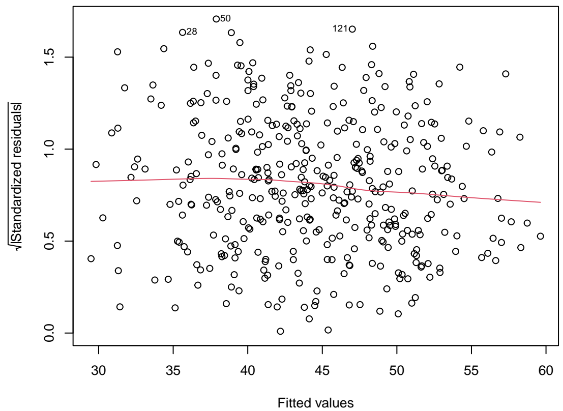
Scale-Location (Option 2) Scale-Location
