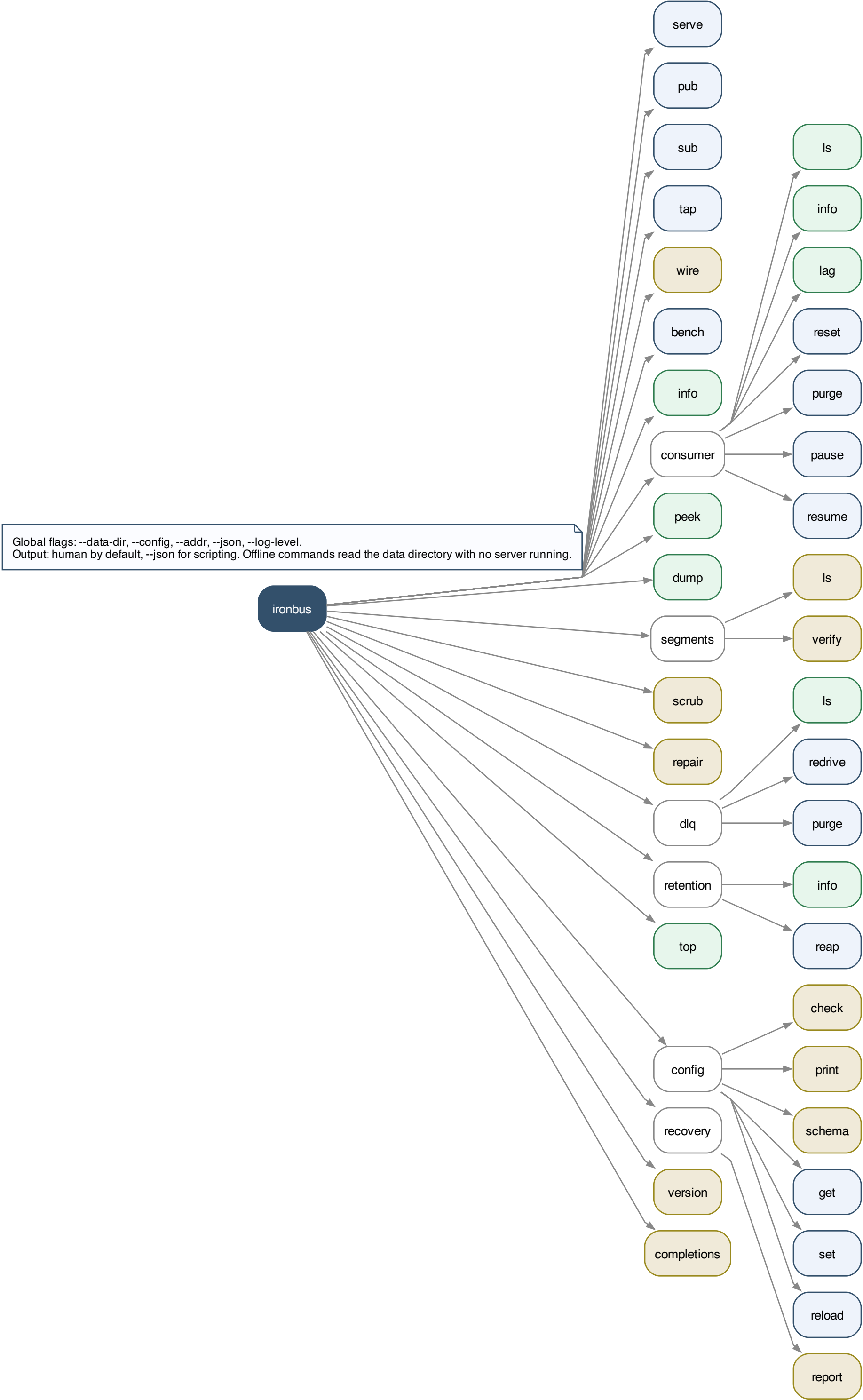
IronBus CLI command map (one binary = broker + CLI). Green=offline-capable on the data dir, blue=online, tan=offline-only
