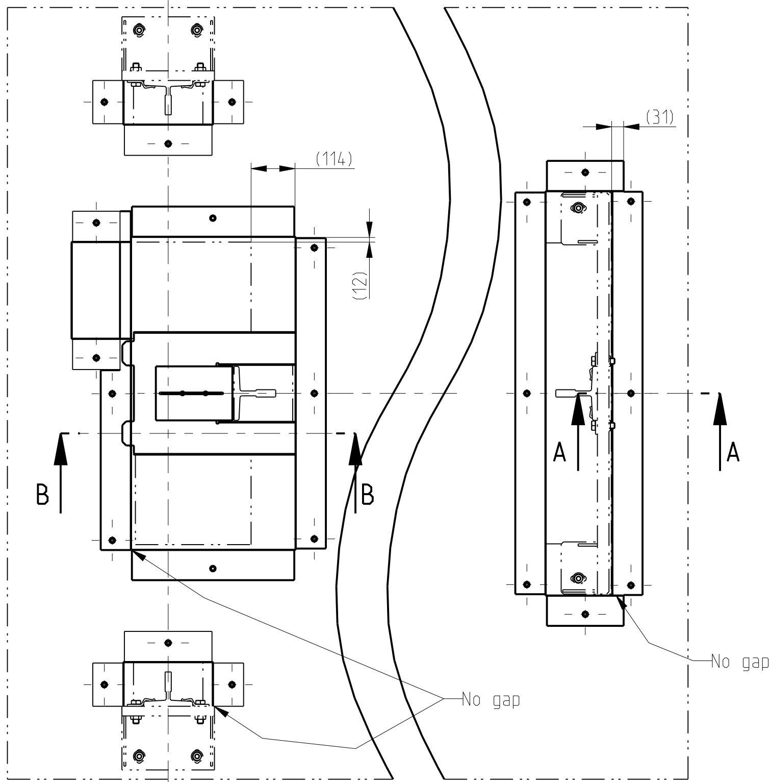
Car Guides Enclosure
