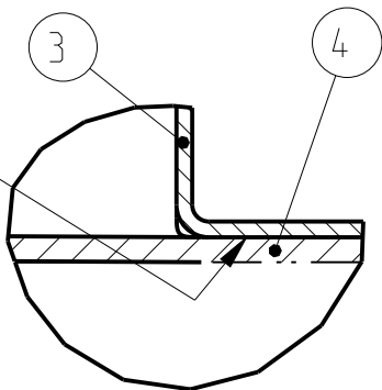
Detail D Scale 1:1
