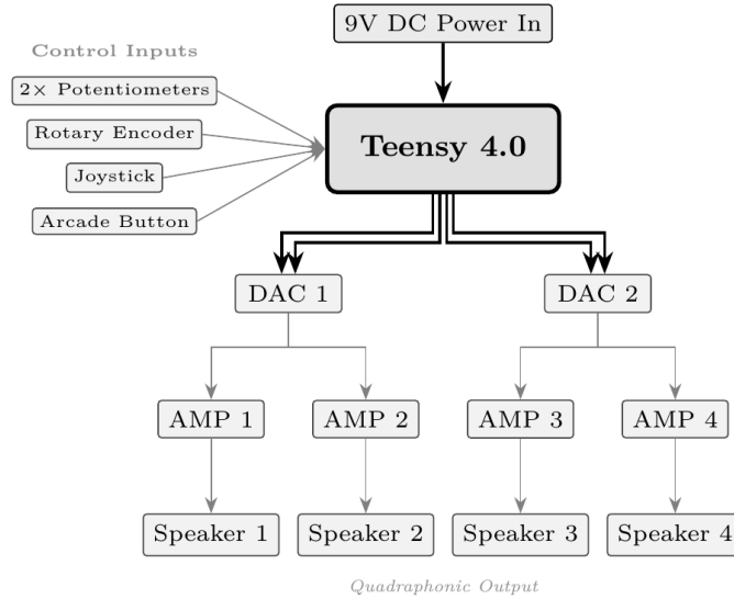
Figure 8: BOUBA hardware architecture.
