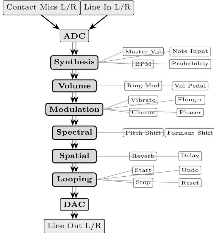
Figure 4: NEPTR’s signal flow and menu structure.
