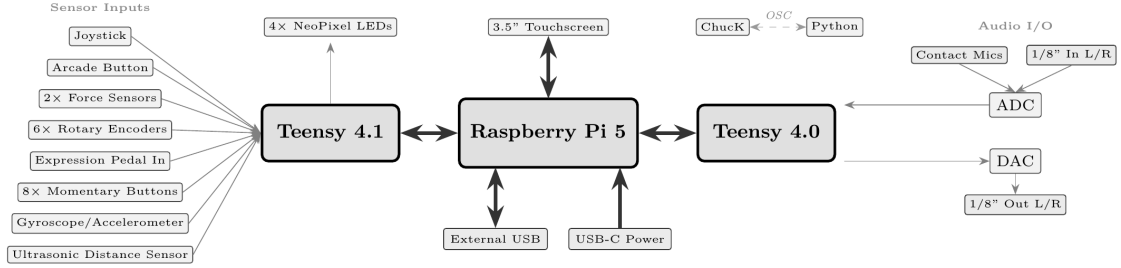
Figure 3: NEPTR’s hardware architecture.
