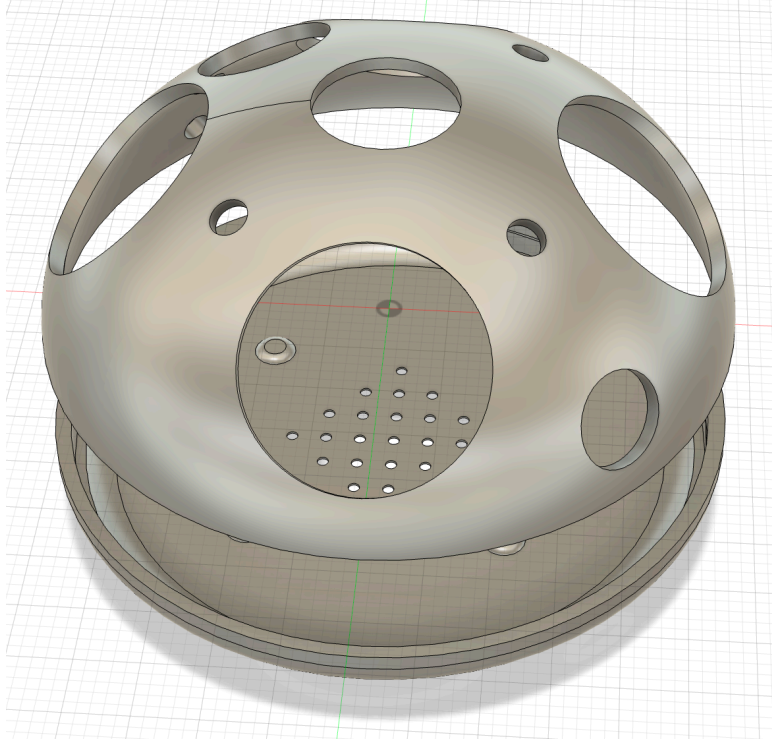
Figure 9: BOUBA 3D-printed enclosure.
