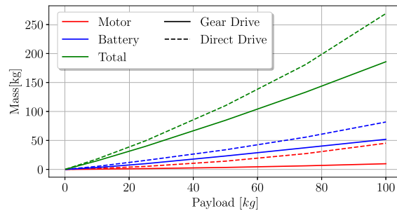
Fig. 12. Effect of the gearbox on the evolution of the components' masses (for a given endurance of 15 min).
