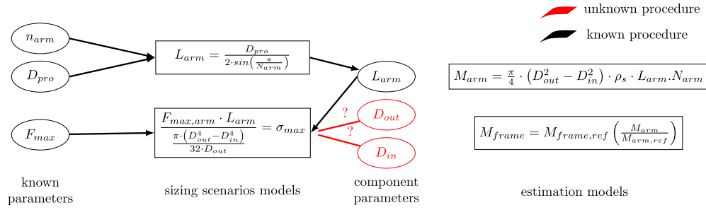
Fig. 5. Design Graph for the frame selection (in red underconstraint).
