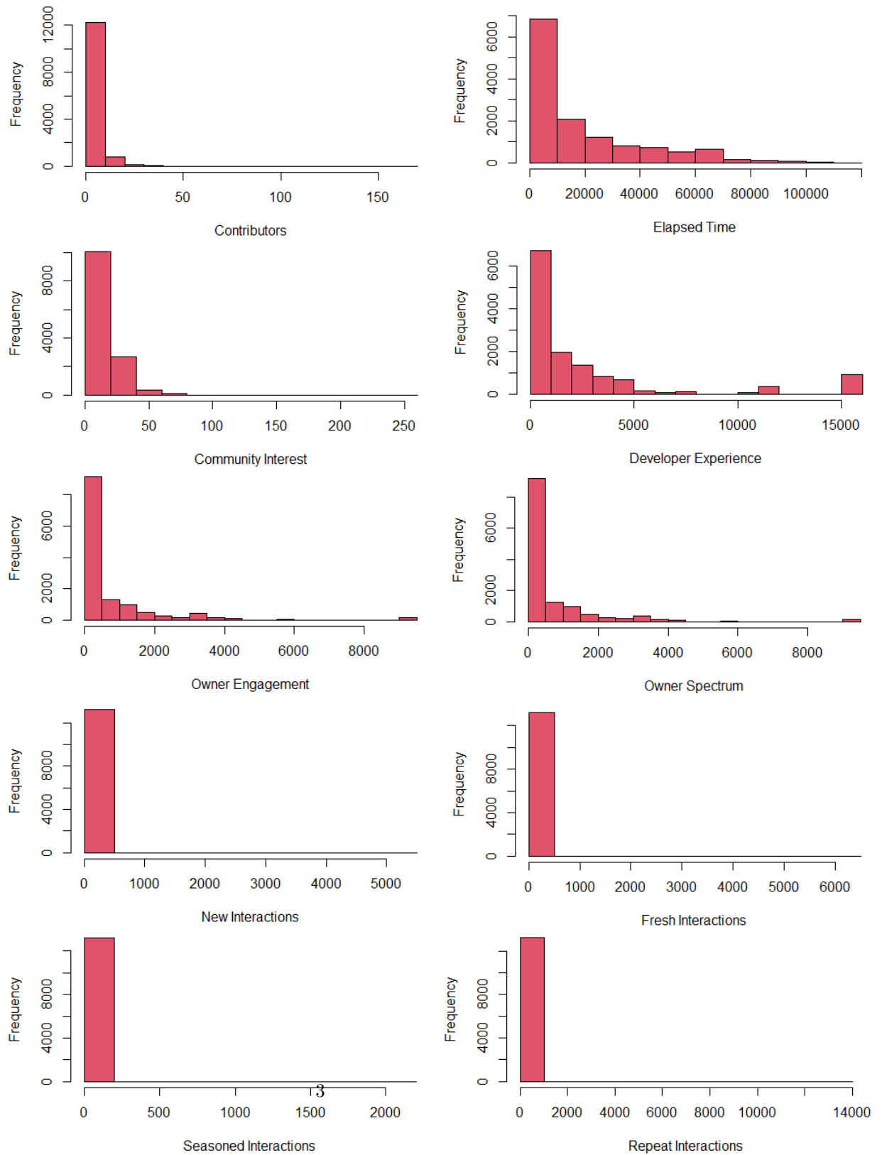
Figure 2: Distributions of Eclipse Model Variables
