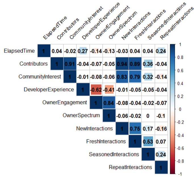
Figure 4: Correlation matrix of variables: Android
