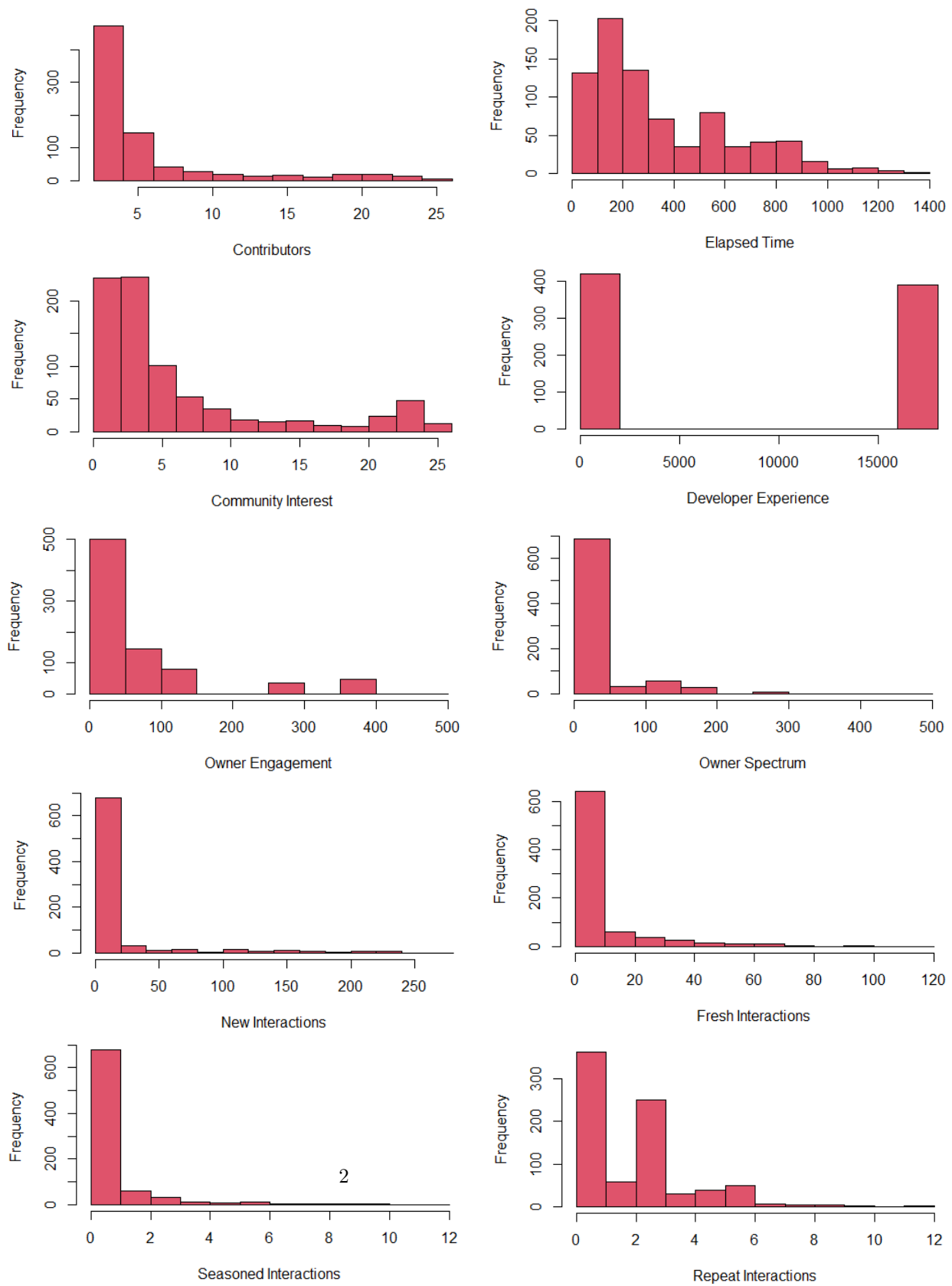
Figure 1: Distributions of Android Model Variables
