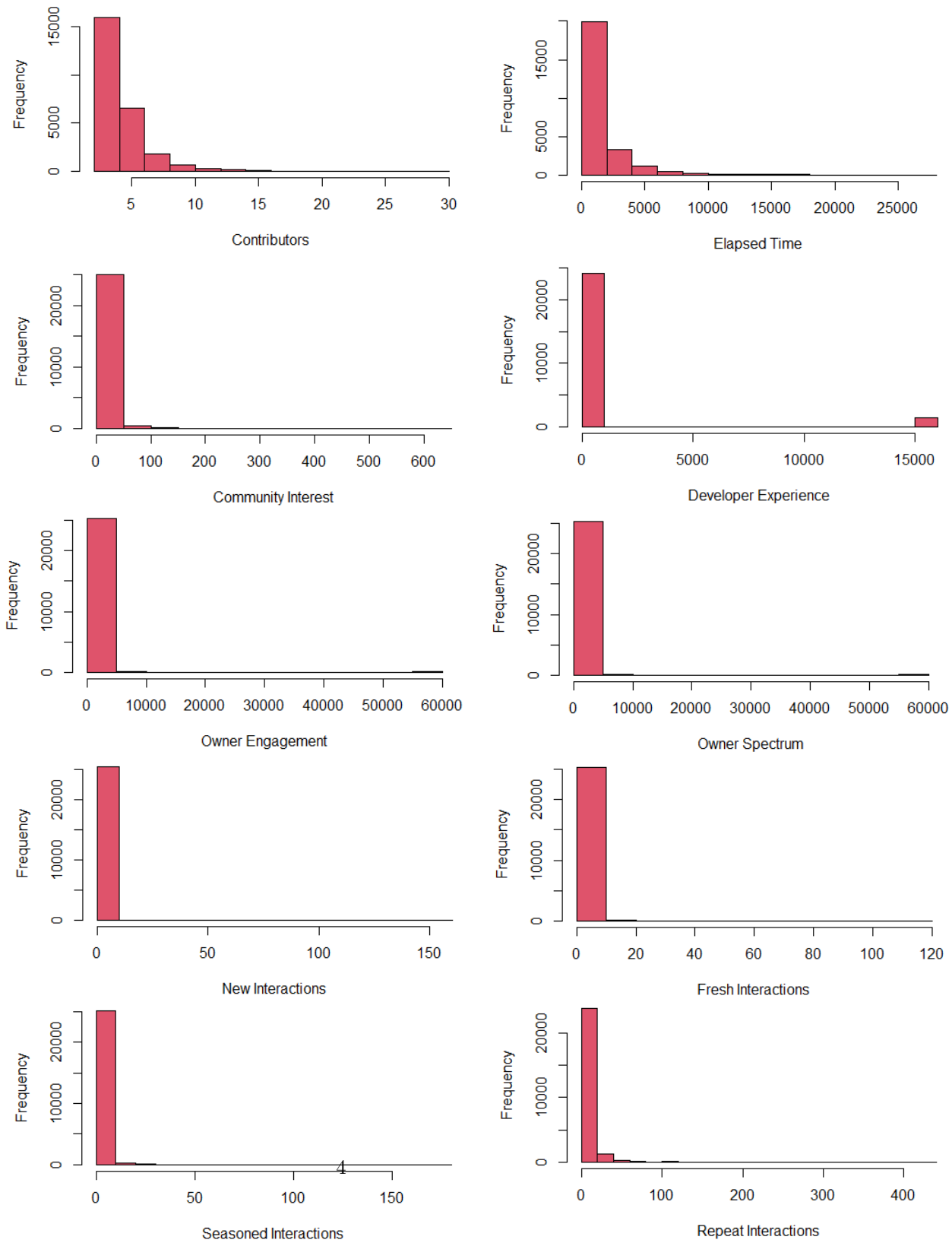
Figure 3: Distributions of OpenStack Model Variables
