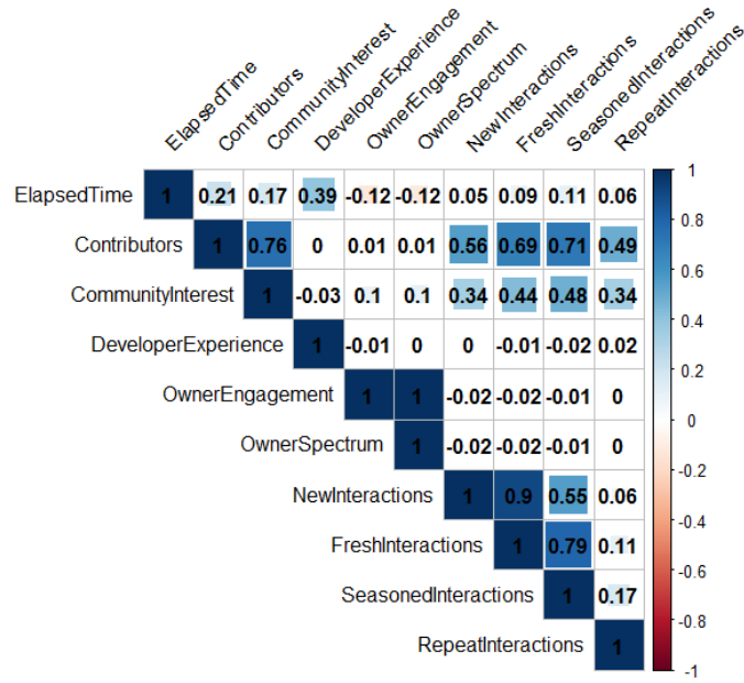
Figure 5: Correlation matrix of variables: Eclipse
