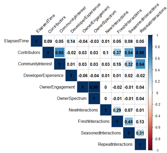
Figure 6: Correlation matrix of variables: OpenStack
