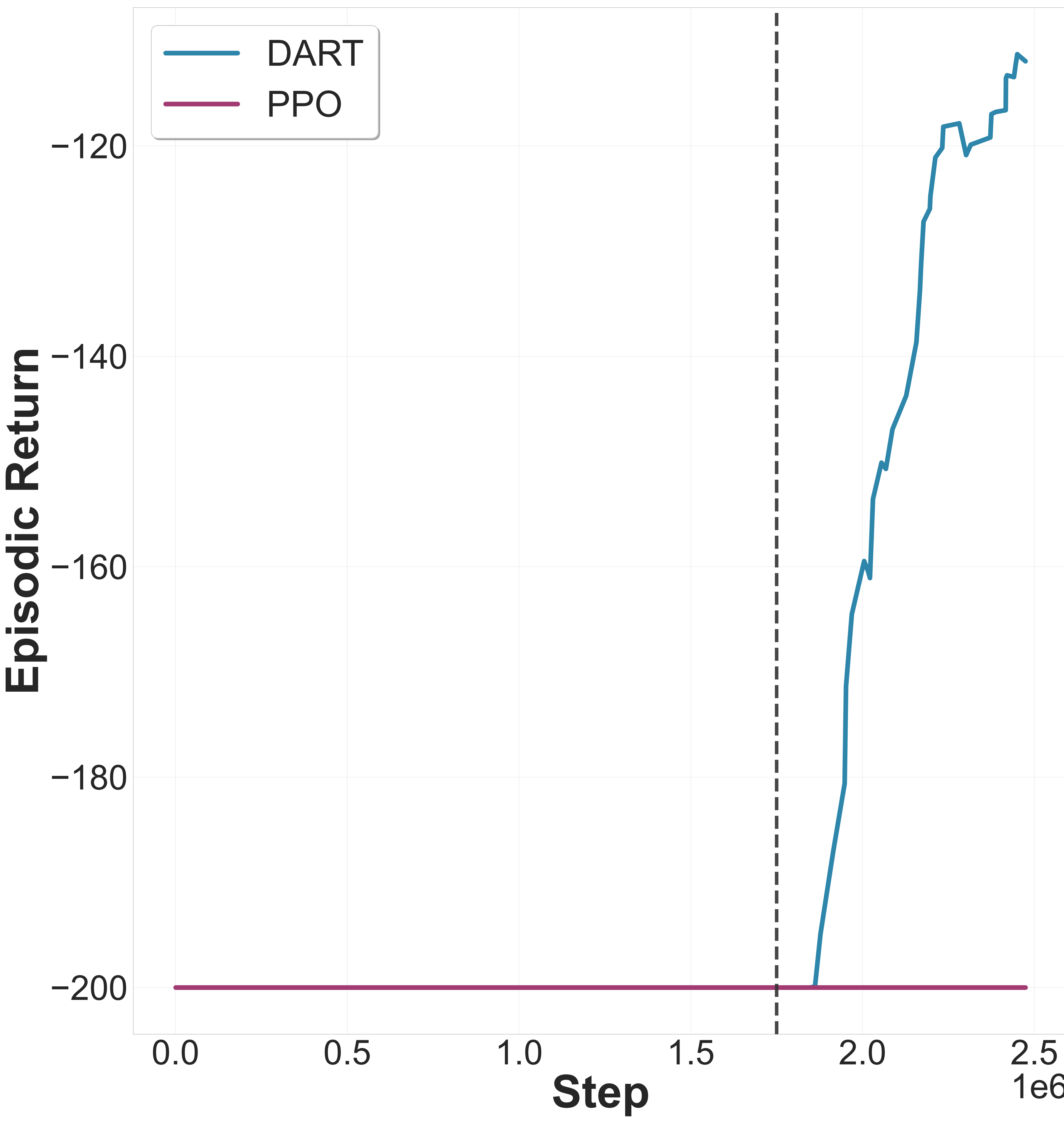
MountainCar-v0
