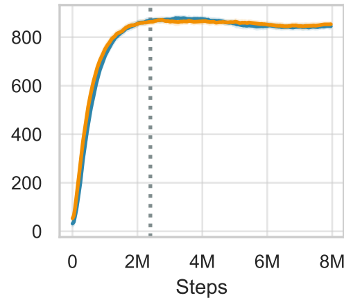
ball_in_cup-catch
