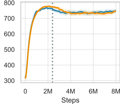
cartpole-balance
