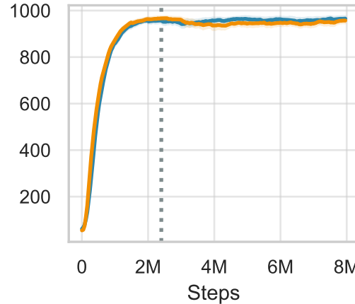
cartpole-balance_sparse
