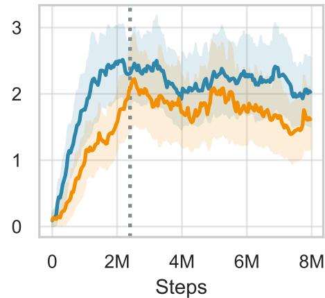
acrobot-swingup_sparse
