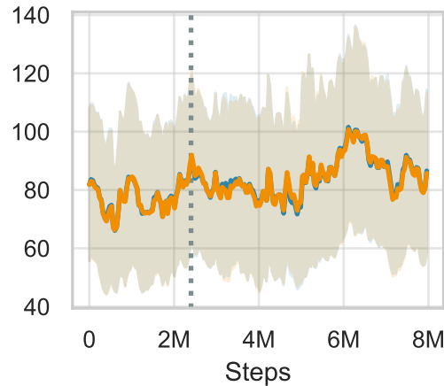
manipulator-insert_peg
