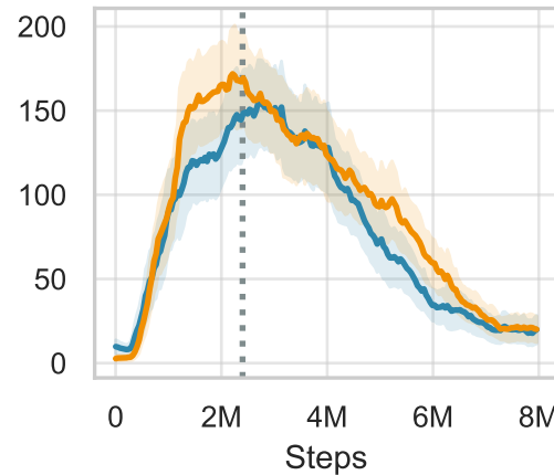
point_mass-hard
