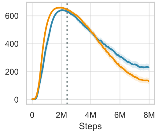
point_mass-easy
