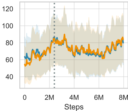
manipulator-insert_ball
