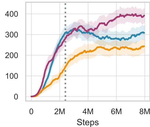
cartpole-swingup_sparse
