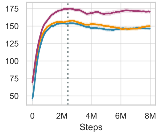
cartpole-three_poles
