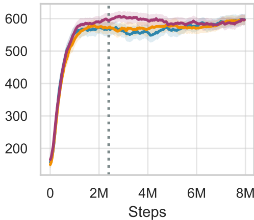
cartpole-swingup
