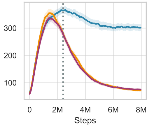
cheetah-run
