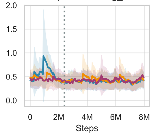
manipulator-bring_ball
