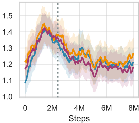
humanoid-walk
