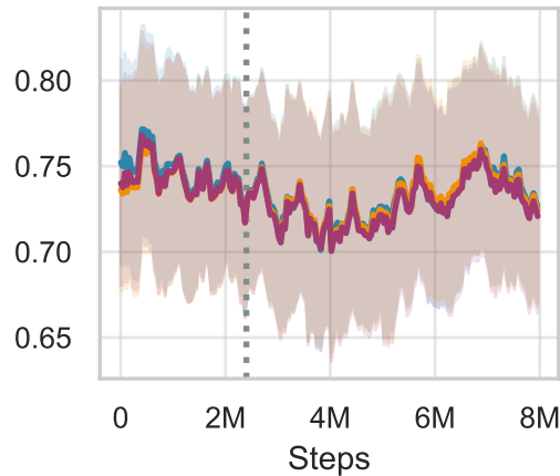
humanoid_CMU-run
