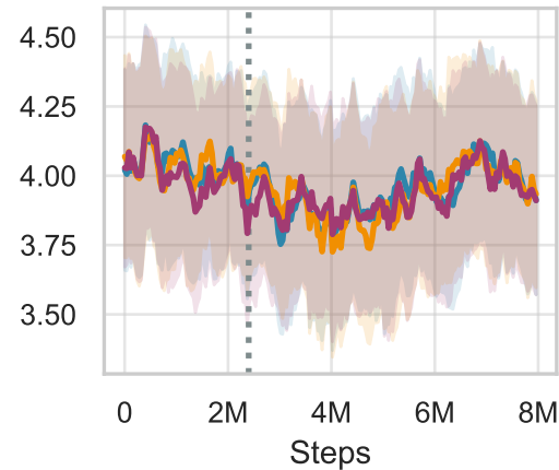
humanoid_CMU-stand
