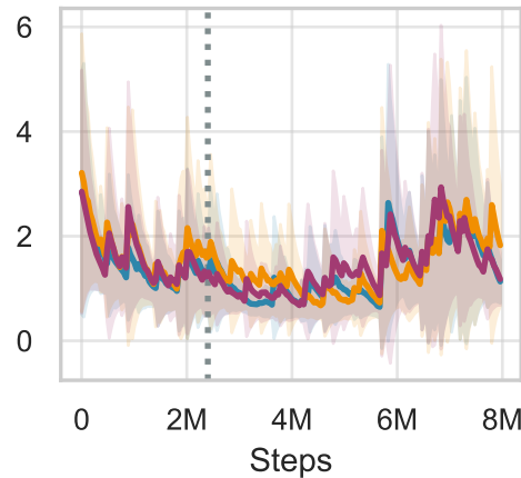
manipulator-bring_peg
