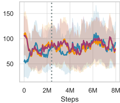
manipulator-insert_peg
