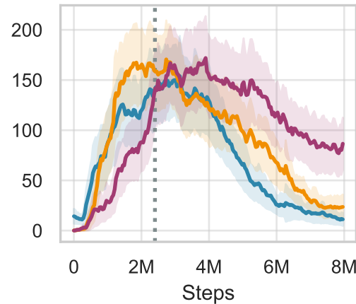
point_mass-hard
