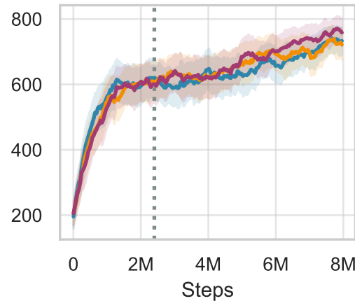
reacher-easy
