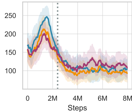
quadruped-walk
