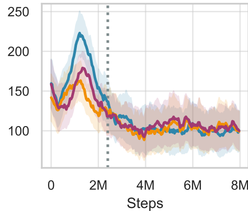
quadruped-run
