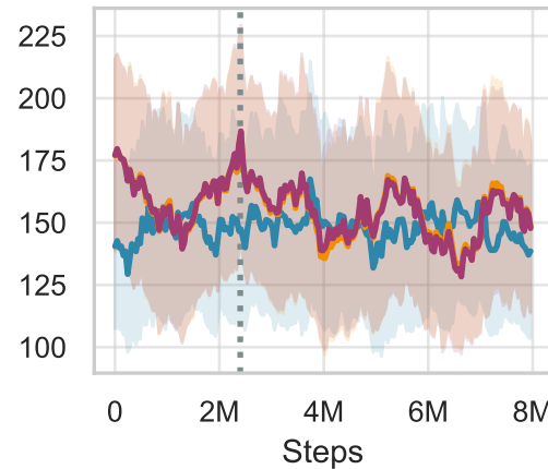
swimmer-swimmer15
