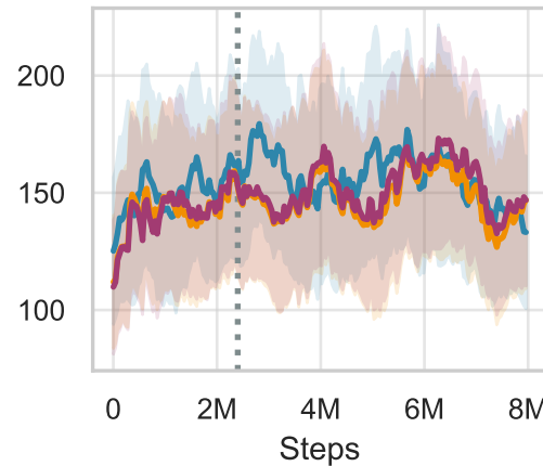
swimmer-swimmer6
