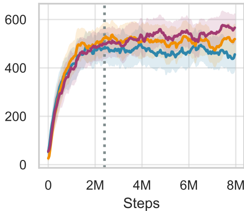
reacher-hard
