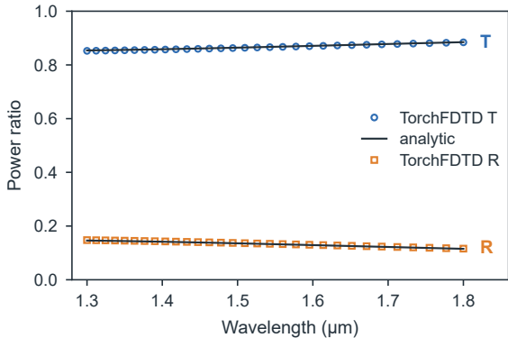
a Slab transmission and reflection, 31 samples
