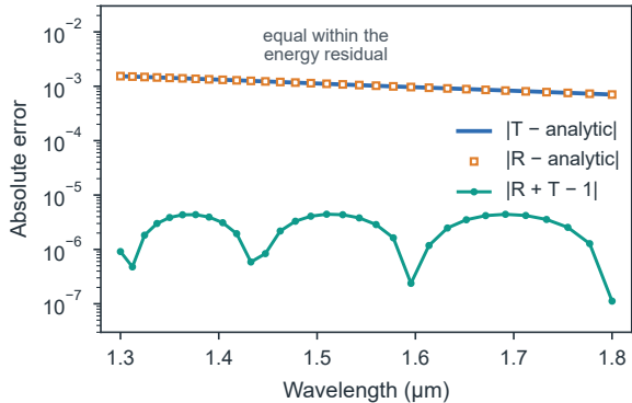
b Error against the analytic spectra and energy residual
