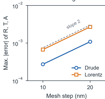
d Mesh convergence
