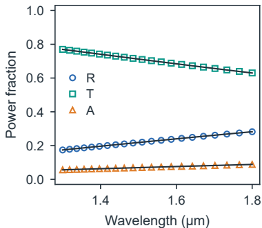
b Drude slab, 0.1\ \mu\text{m}
