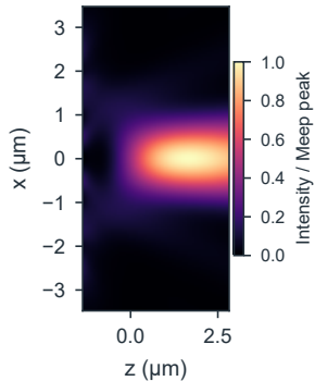
c Meep, |E|^2
