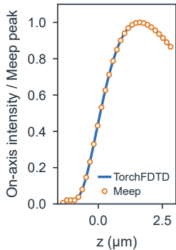
d On-axis intensity
