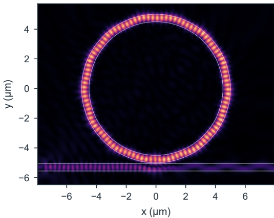
c Bus transmission, 89 219 steps
