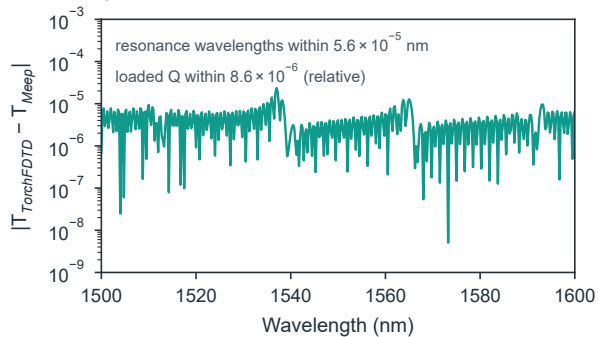
d Solver difference
