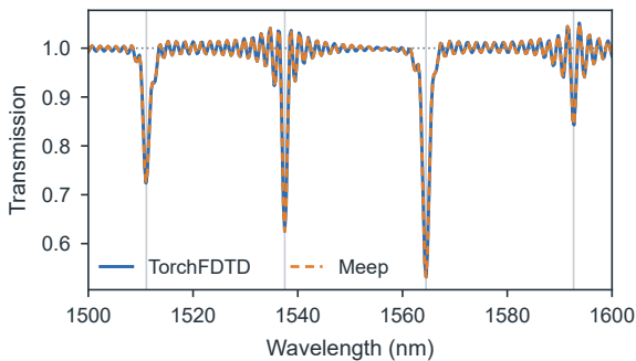
c Bus transmission, 89 219 steps
