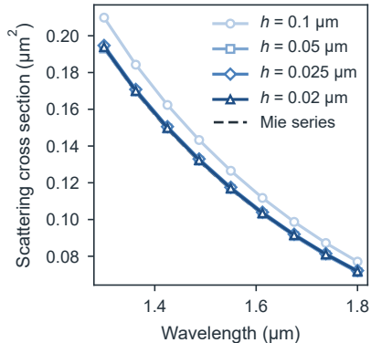
b Cross section by mesh step
