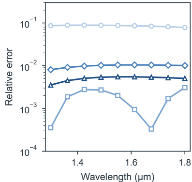
c Relative error against the Mie series
