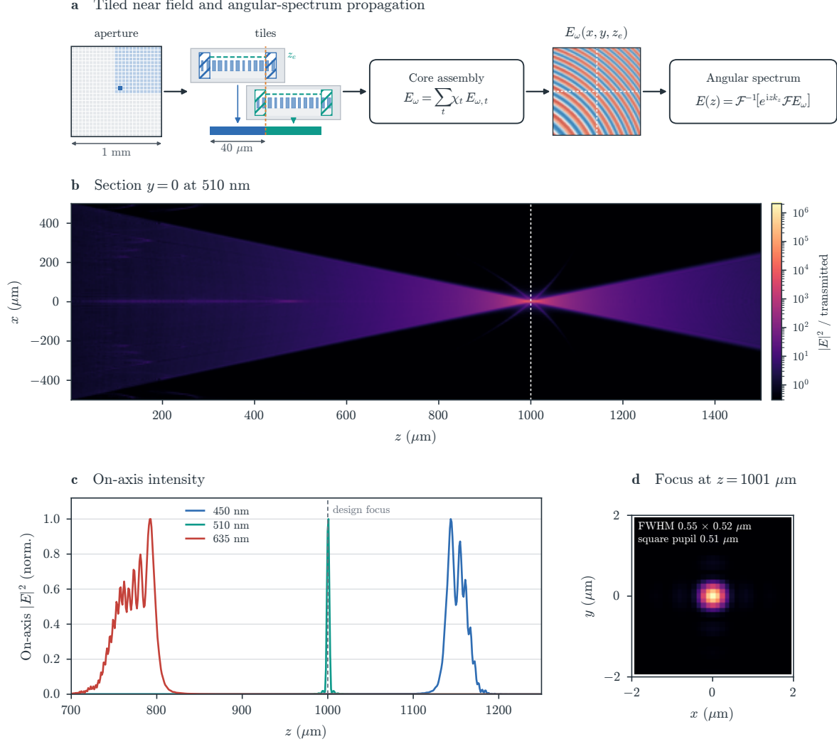
Figure 12: A 1 \text{ mm} \times 1 \text{ mm} silicon nitride metalens evaluated with overlapping tiles on one RTX 5880 Ada of 48 GB. (a) Evaluation chain. Tiles of 40 \mu\text{m} cover the shaded quadrant of the aperture, each with its own absorbers (grey) and overlaps (hatched). The cores of their exit-plane fields are assembled, mirrored across x = 0 and y = 0 and propagated with Eq. (4). The assembled field is shown as the real part of E_x at 510 nm around a corner where four tiles meet, with the tile boundaries dashed. (b) Intensity in the plane y = 0 at 510 nm relative to the intensity transmitted just behind the lens, with the design focal length dashed. (c) On-axis intensity at 450, 510 and 635 nm, each normalized to its maximum. (d) Focal spot at 510 nm with its full widths and the full width of a square pupil of the same numerical aperture.
