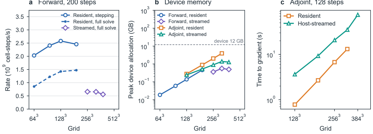
Figure 9: Scaling with grid size on one RTX 3060 of 12 GB. (a) Forward rate in cell-steps per second over 200 steps: the stepping loop and the complete solve of the resident path, and the complete host-streamed solve. (b) Median peak Torch device allocation of the forward and adjoint modes. (c) Median time to gradient of the dielectric adjoint fixture with 128 steps and two checkpoints. Each point is the median of three warmed repetitions.
