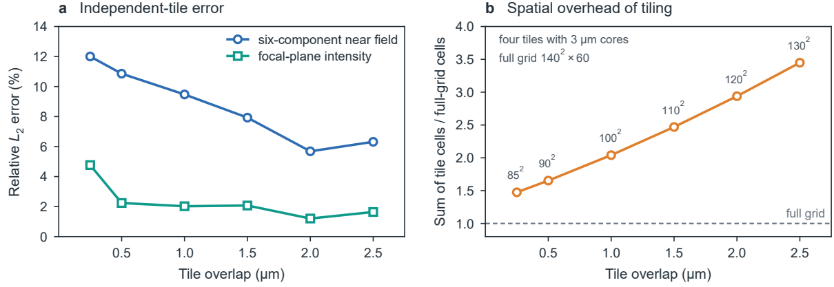
Figure 13: Independent overlapping tiles on an RTX 3060, compared with the full-domain solution. (a) Relative L_2 errors of the six-component near field and the focal-plane intensity with hard core assembly. (b) The summed cell count of all tiles relative to the full grid, including repeated overlap regions, with the tile edge length in cells.
