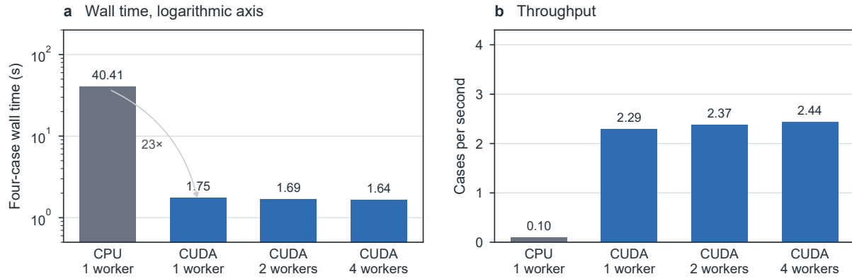
Figure 14: Wall time on a logarithmic axis (a) and throughput (b) of four-structure ensembles on an A100. The CPU bar is one NumPy worker on the four-core host of that container. Bars are medians of three measured batches after warm-up.
