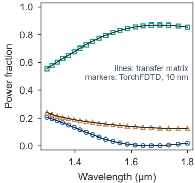
b Two-pole Lorentz slab, 0.5 \mu\text{m}
