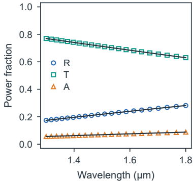
a Drude slab, 0.1 \mu\text{m}
