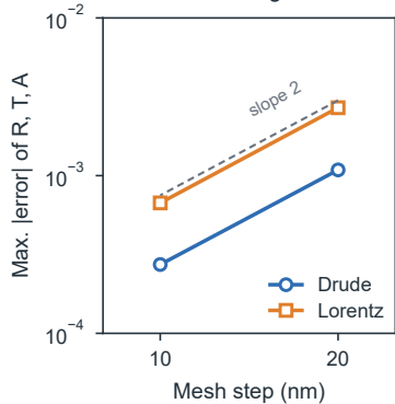
c Mesh convergence
