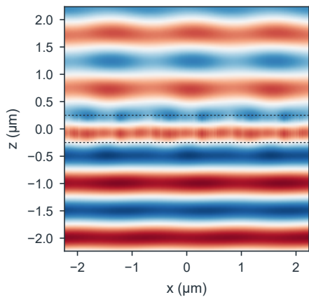
d Initial design, \text{Re } E_x at 1.00 \mu\text{m}
