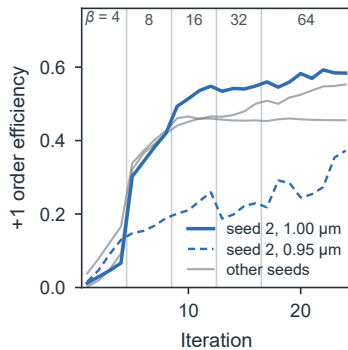
b Objective history
