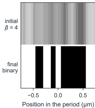
a Design density
