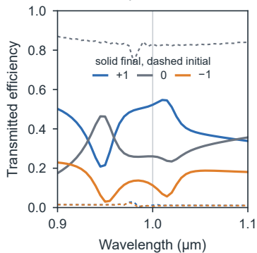
c Order spectra
