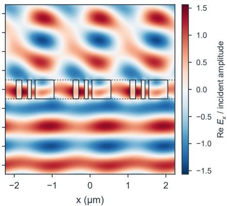
e Final binary design, \text{Re } E_x at 1.00 \mu\text{m}
