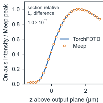
c On-axis intensity
