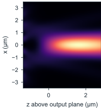
a TorchFDTD, |E|^2 at 1.55\ \mu\text{m}
