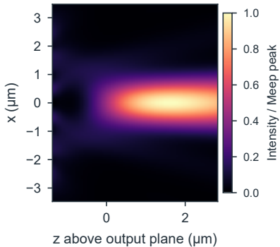
b Meep, |E|^2 at 1.55\ \mu\text{m}
