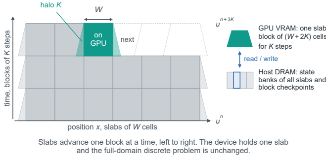
Figure 1: Execution and differentiation in TorchFDTD. (a) The forward map from design parameters to an objective evaluated after angular-spectrum propagation, and its transposed chain. Every forward kernel has its own transpose kernel, and the transposed sweep obtains forward states from checkpoint replay. (b) Host-streamed execution sweeps causal slabs of W cells with halos of K cells over blocks of K steps. One slab block resides on the GPU while the state banks of all slabs and the block checkpoints stay in host DRAM. (c) Independent lateral tiles solve overlapping subdomains with their own absorbers and assemble the core fields on the output plane. Coupling across the artificial cut is lost, and the resulting error is measured against a full-domain solution.
