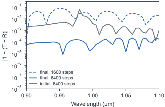
a Energy balance, 25 nm mesh
