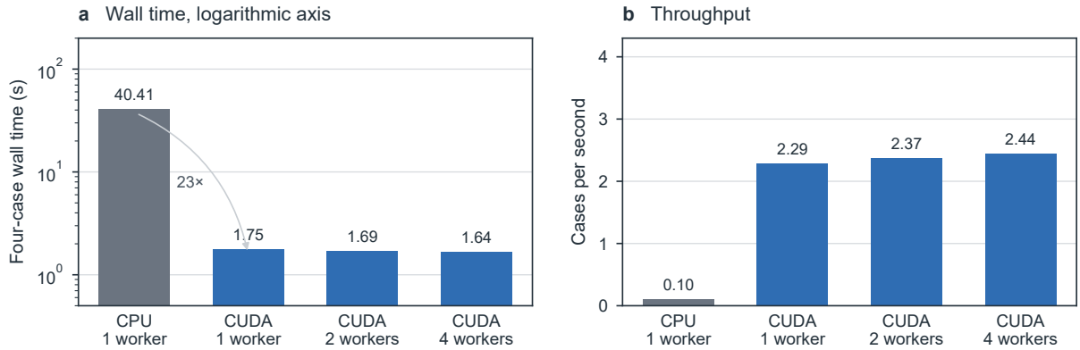
Figure 13: Wall time on a logarithmic axis (a) and throughput (b) of four-structure ensembles on an A100. The CPU bar is one NumPy worker on the four-core host of that container. Bars are medians of three measured batches after warm-up.
