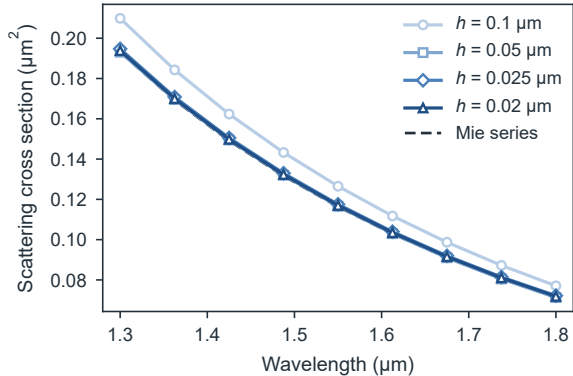
a TFSF sphere cross section by mesh step
