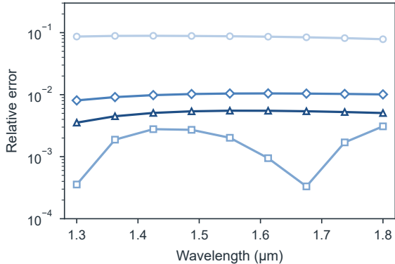
b Relative error against the Mie series
