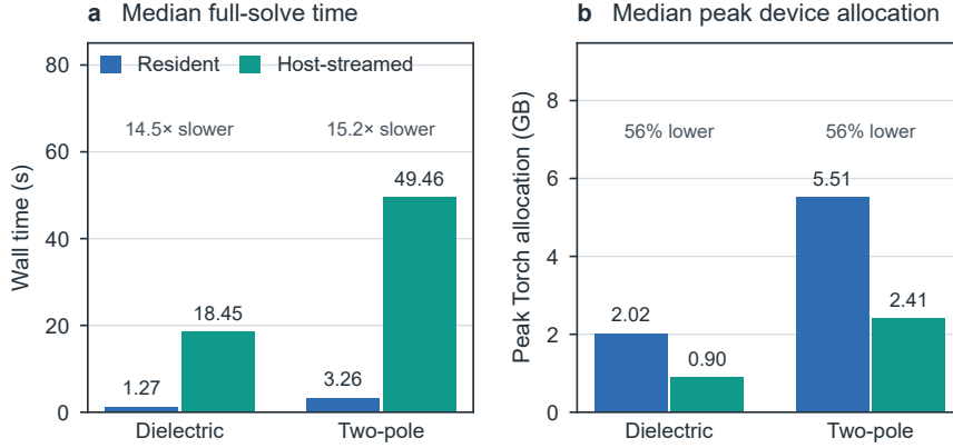
Figure 6: Memory–time trade-off between GPU-resident and host-streamed adjoints on an A100 80GB PCIe in a four-core container. Matched 256^3 grids use 128 steps and two checkpoints. (a) Median full-solve time. (b) Median peak Torch device allocation, which excludes the CUDA context and non-Torch allocations. Both quantities use three interleaved warmed repetitions. GB denotes 10^9 bytes.
