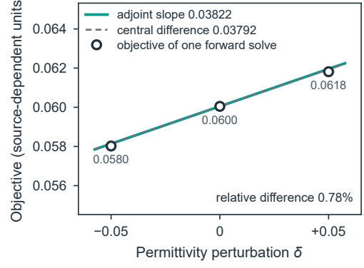
Figure 7: Streamed evaluation of the fixed 44\ \mu\text{m} pillar-array objective on an RTX 3060. (a) Timeline of the recorded driver: the forward pass, the adjoint sweep, the two central-difference (FD) forward solves and the remaining setup and checks. (b) The objective at the unperturbed and the two perturbed permittivities of the central pillar region. The adjoint directional derivative and the central-difference secant are drawn as slopes through the unperturbed value. Both use the same sampled output plane and propagation model.
