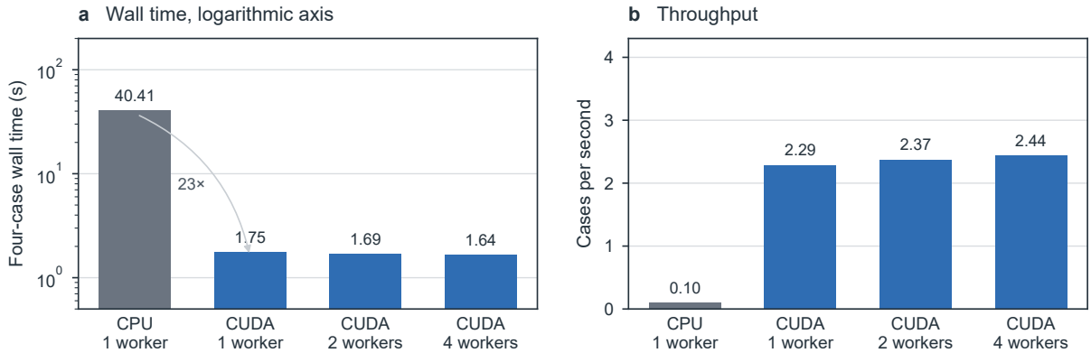
Figure 5: Wall time on a logarithmic axis (a) and throughput (b) of four-structure ensembles on an A100. The CPU bar is one NumPy worker on the four-core host of that container. Bars are medians of three measured batches after warm-up.
