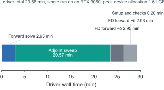
Figure 7: Streamed evaluation of the fixed 44\ \mu\text{m} pillar-array objective on an RTX 3060. (a) Timeline of the recorded driver: the forward pass, the adjoint sweep, the two central-difference (FD) forward solves and the remaining setup and checks. (b) The objective at the unperturbed and the two perturbed permittivities of the central pillar region. The adjoint directional derivative and the central-difference secant are drawn as slopes through the unperturbed value. Both use the same sampled output plane and propagation model.
