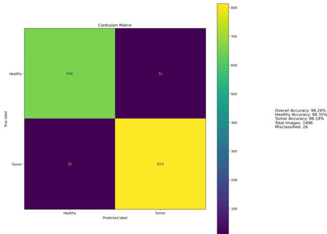
Figure 2. Confusion Matrix
