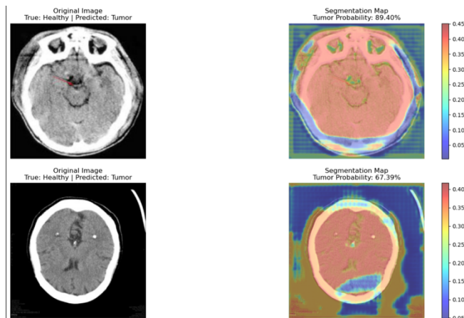
Figure 3. Misclassified examples
