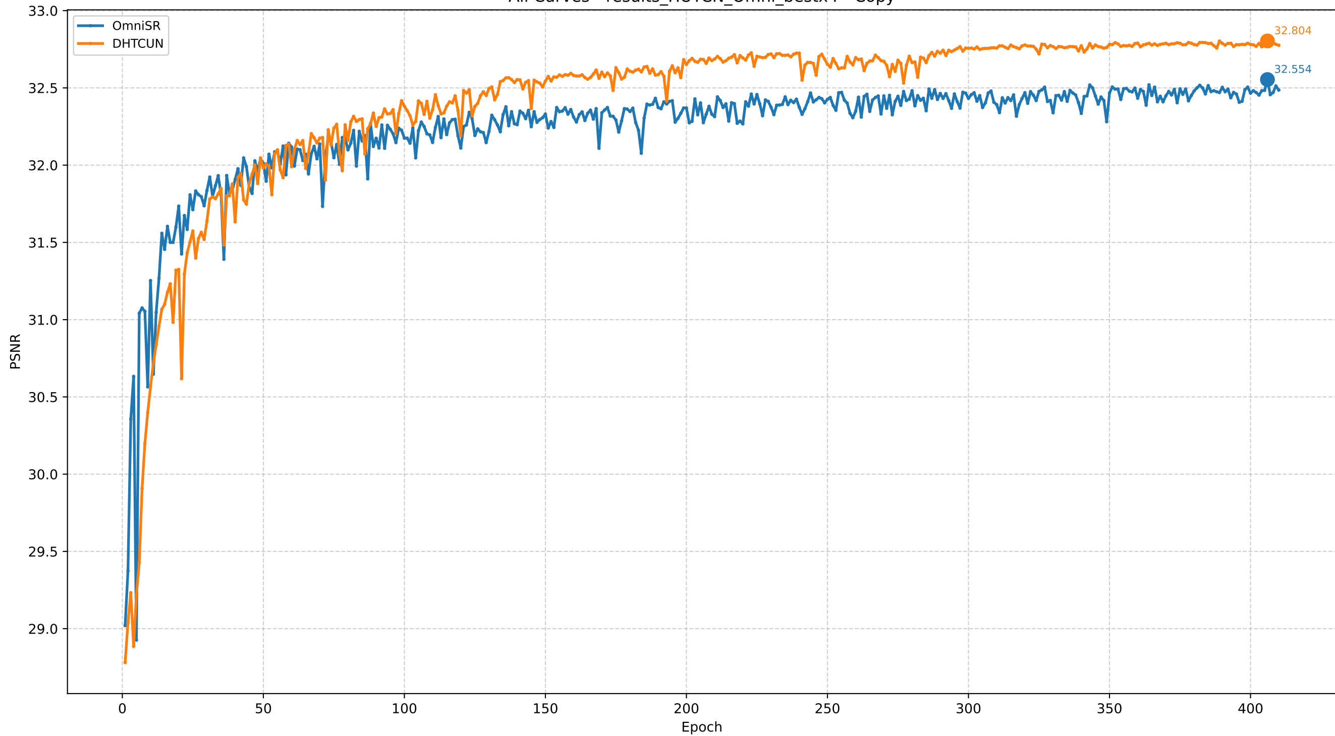
All Curves - results_HUTCN_Omni_bestx4 - Copy
