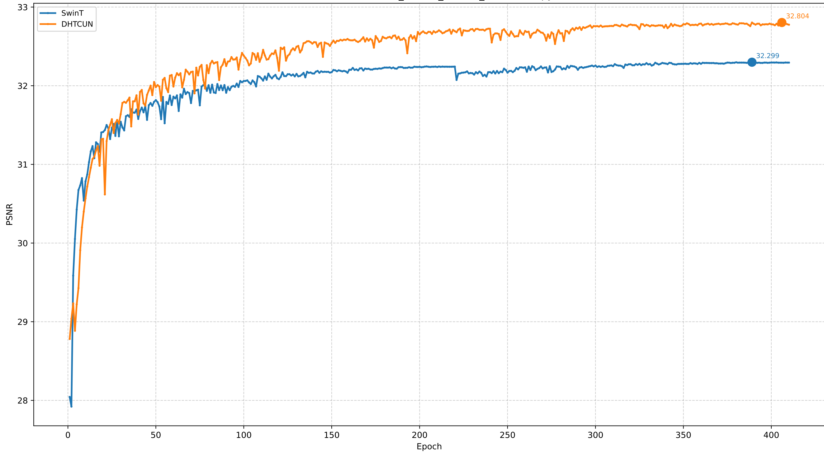
All Curves - results_HUTCN_SwinT2_bestx4 - Copy
