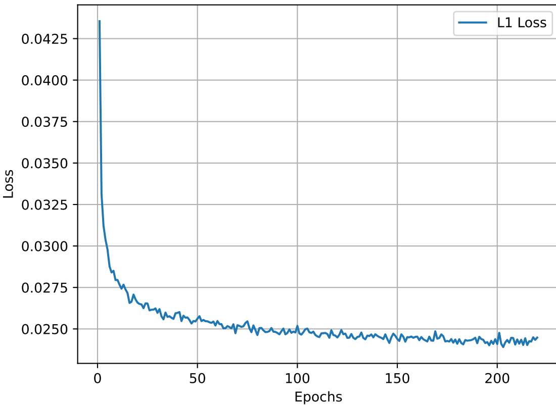
L1 Loss
