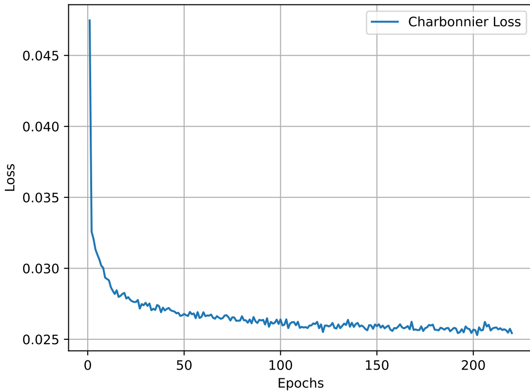
Charbonnier Loss
