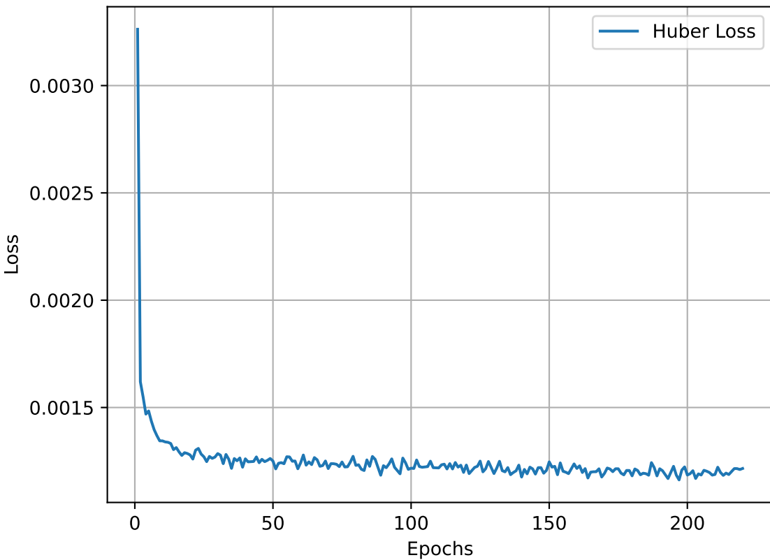
Huber Loss
