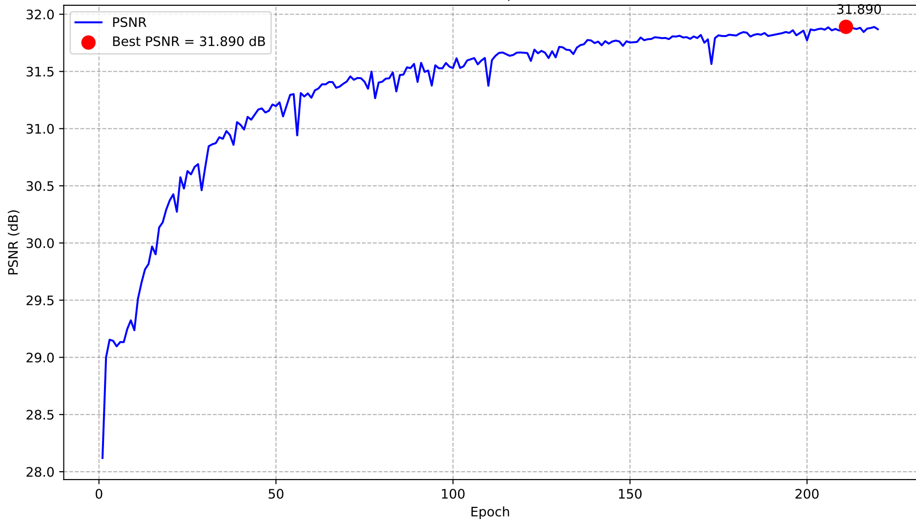
PSNR vs Epochs
