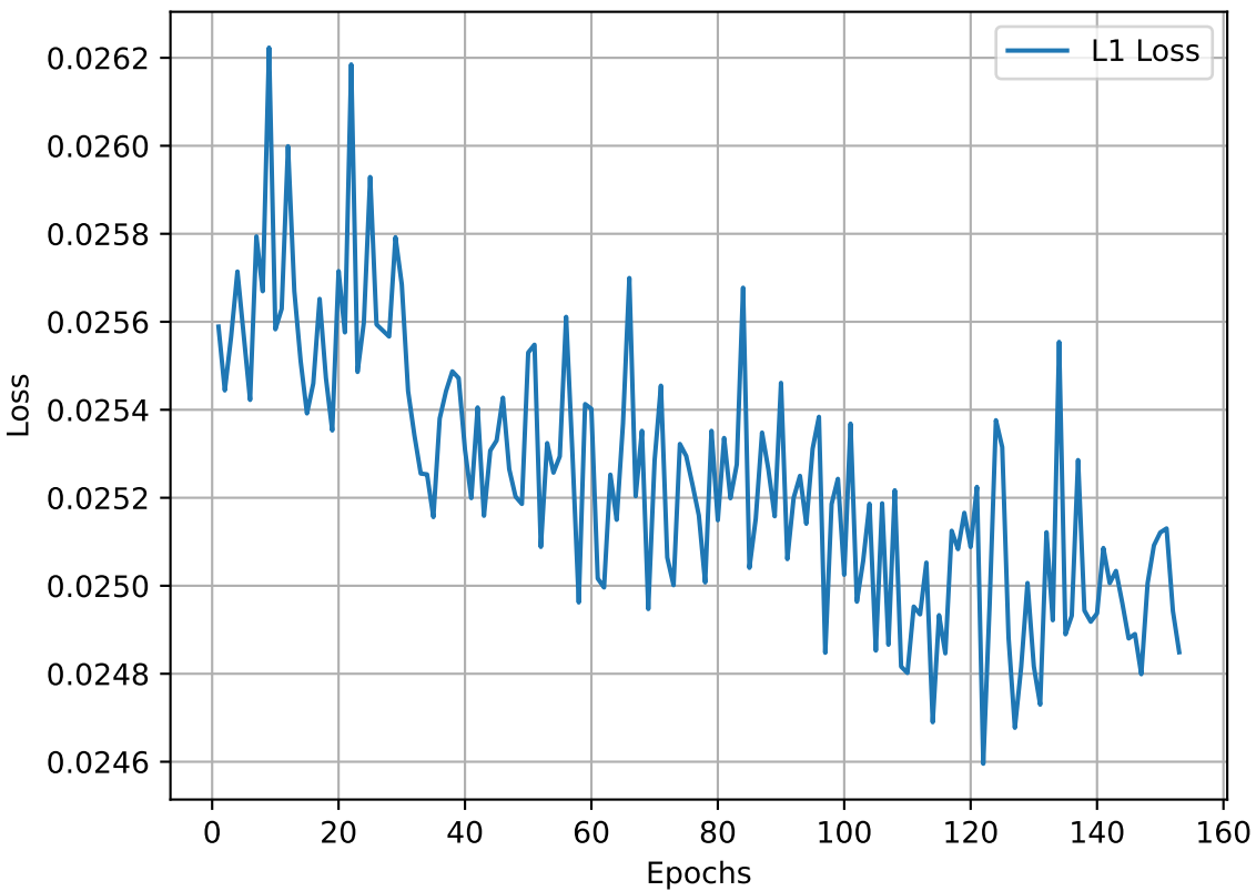
L1 Loss
