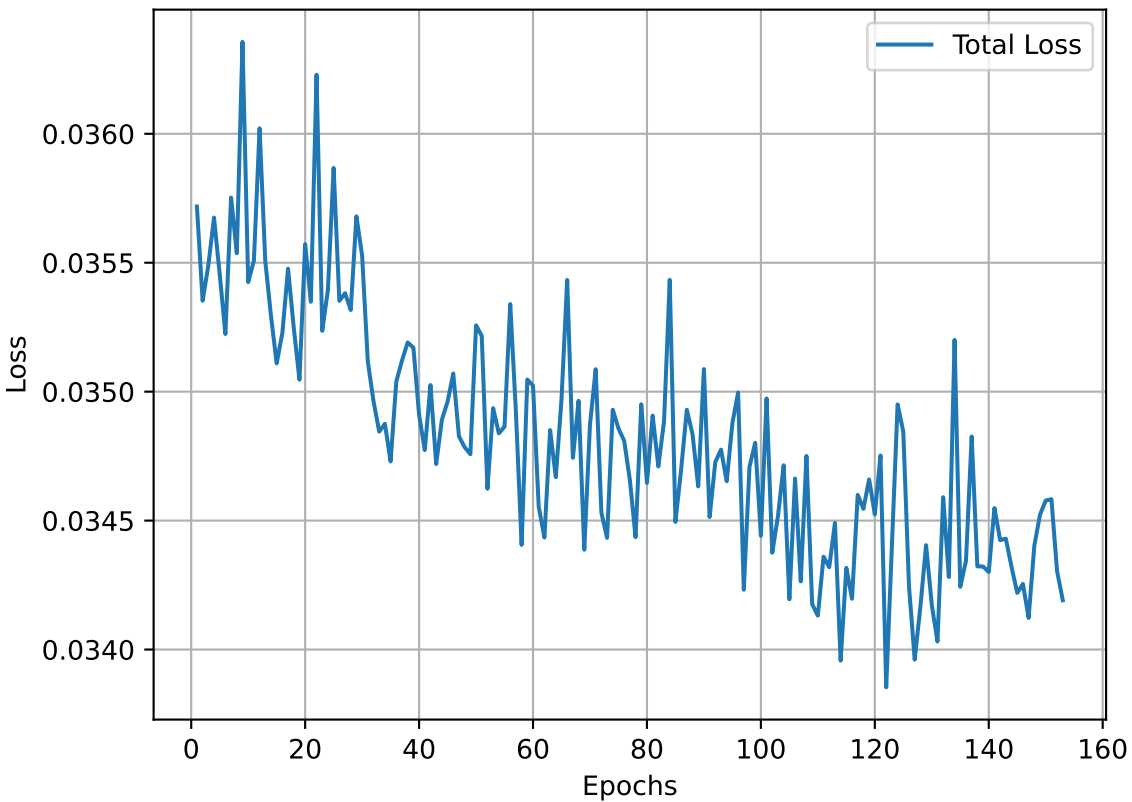
Total Loss
