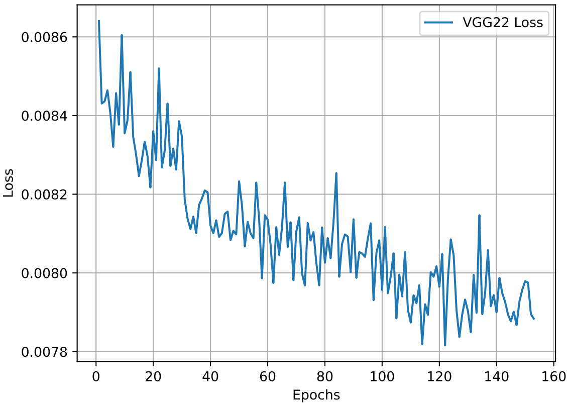
VGG22 Loss
