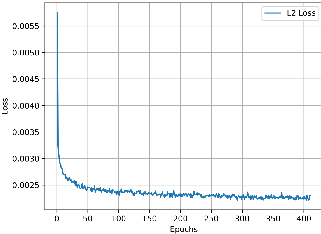
L2 Loss
