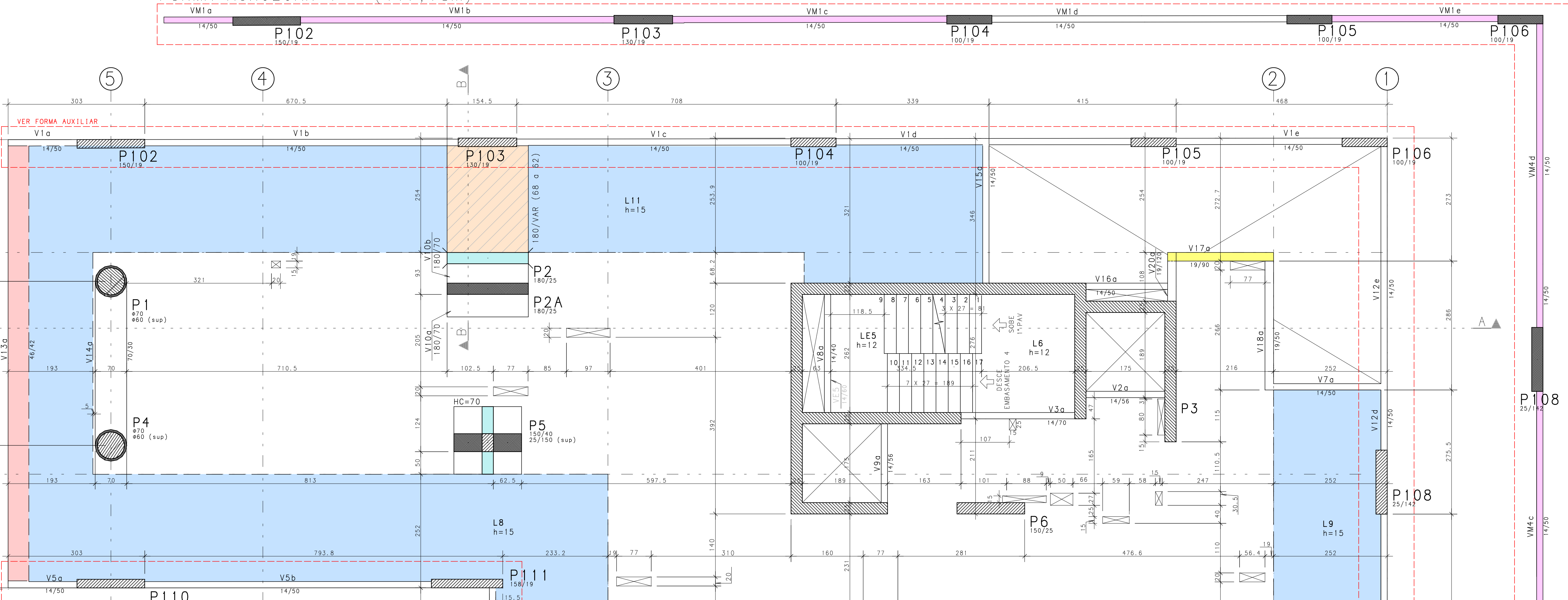
FORMA AUXILIAR 1 - (+17.75m)
