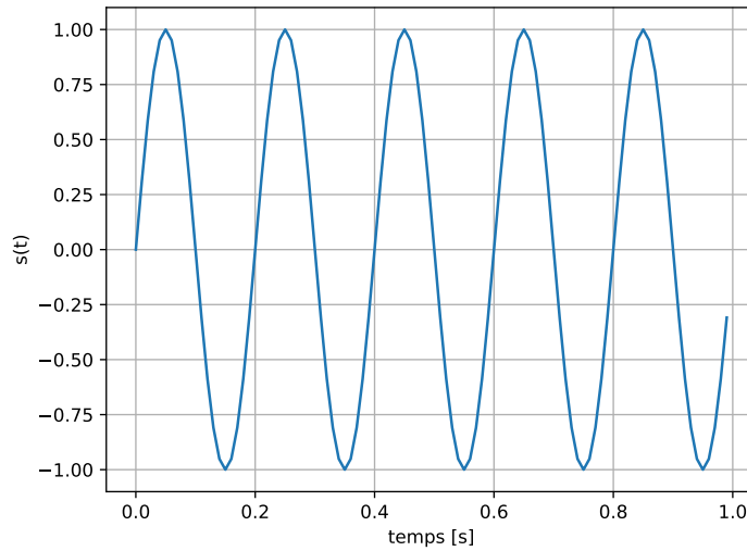
Figure 2.2: Sine wave with frequency f_0 = 5\text{Hz} .
