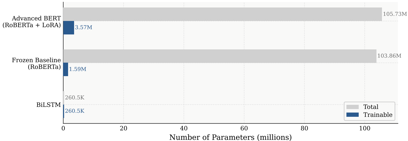
Parameter Counts by Model
