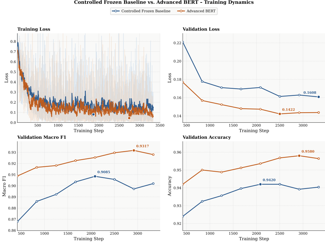
Figure 1: Training dynamics for the controlled frozen baseline (blue) and the advanced BERT (orange). Top left: step-level training loss with raw signal (pale) and EMA-smoothed overlay (solid). Top right: validation loss at fixed evaluation intervals. Bottom left: validation macro F1. Bottom right: validation accuracy. Filled circles with annotations mark the best-checkpoint step for each run.
