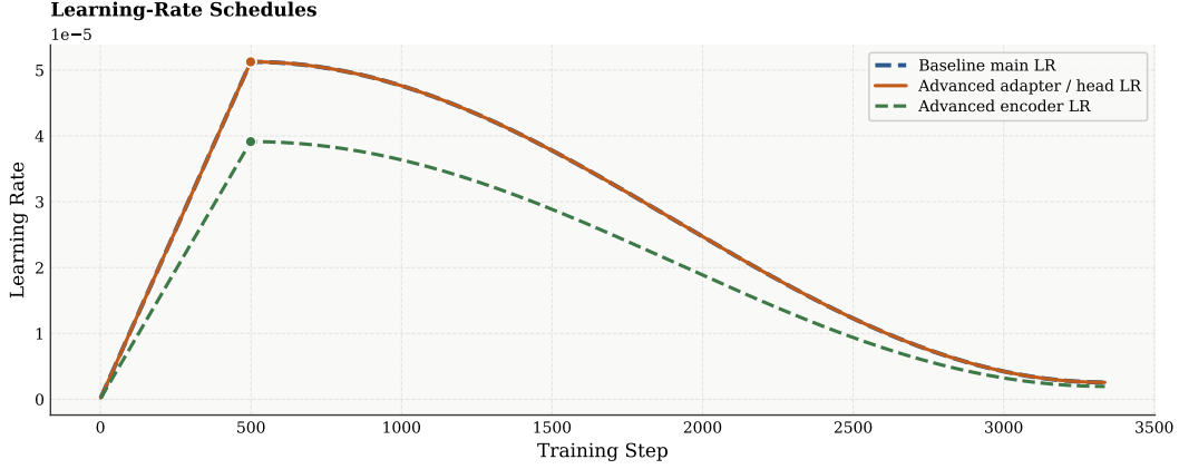
Figure 2: Learning-rate schedules. Blue dashed: main LR for the frozen baseline. Orange solid: adapter and classification-head LR for the advanced BERT. Green dashed: encoder LR for the advanced BERT, held lower to protect pretrained representations. The baseline and advanced adapter schedules are identical, so the dashed baseline trace is intentionally styled to remain visible on top of the solid orange line.
