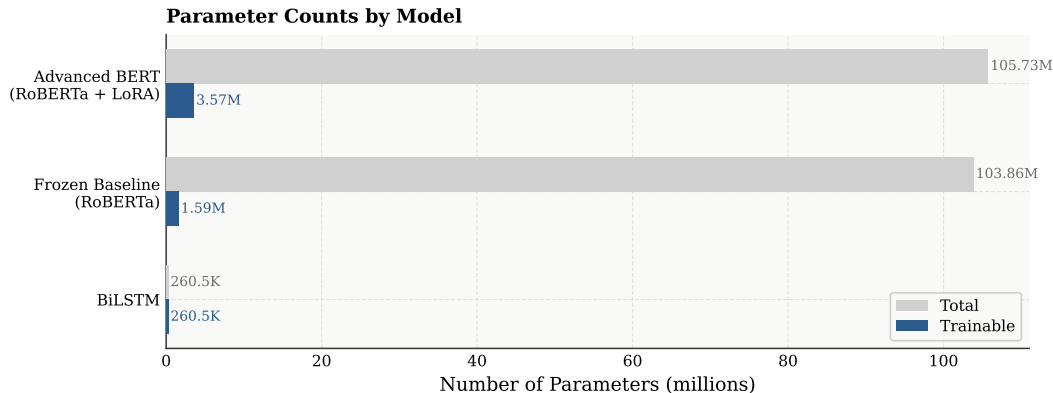
Figure 4: Total (gray) vs. trainable (blue) parameter counts for each model. The BiLSTM is fully trainable but tiny ( \approx 261 K). Both BERT-based models share a \sim 104 – 106 M-parameter backbone; the advanced model activates about 2.2\times more trainable parameters than the frozen baseline by injecting LoRA adapters and enabling BitFit, while keeping the vast majority of the pretrained encoder frozen.
