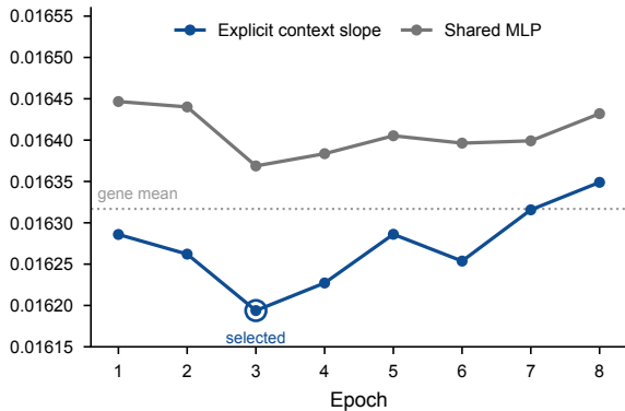
a Validation Huber loss (selection criterion)
