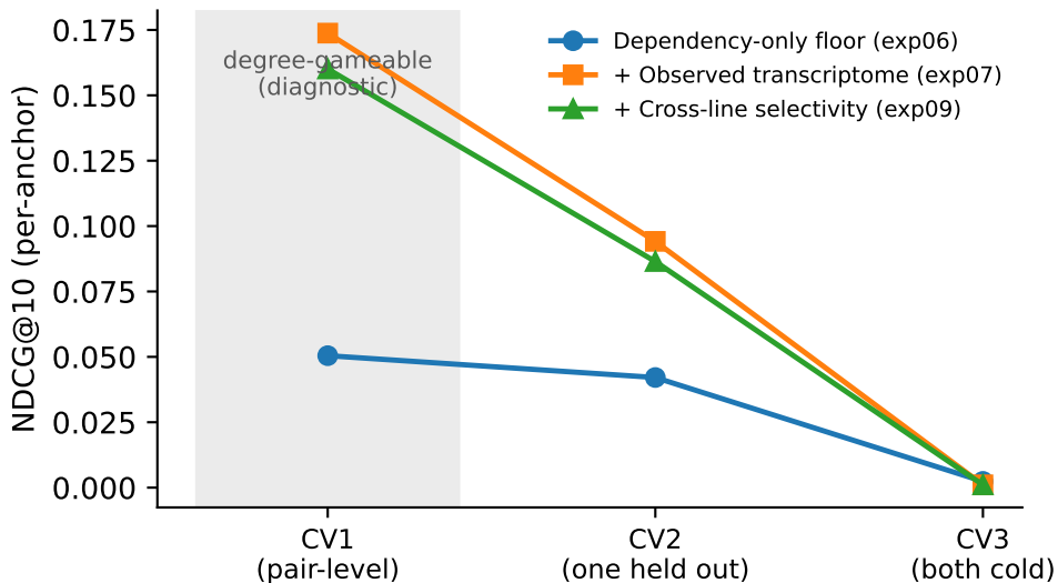
Ranking quality down the cold-start difficulty ladder
