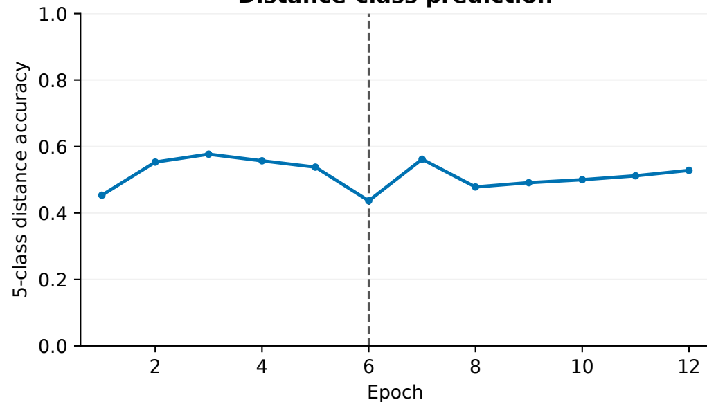
Distance-class prediction
