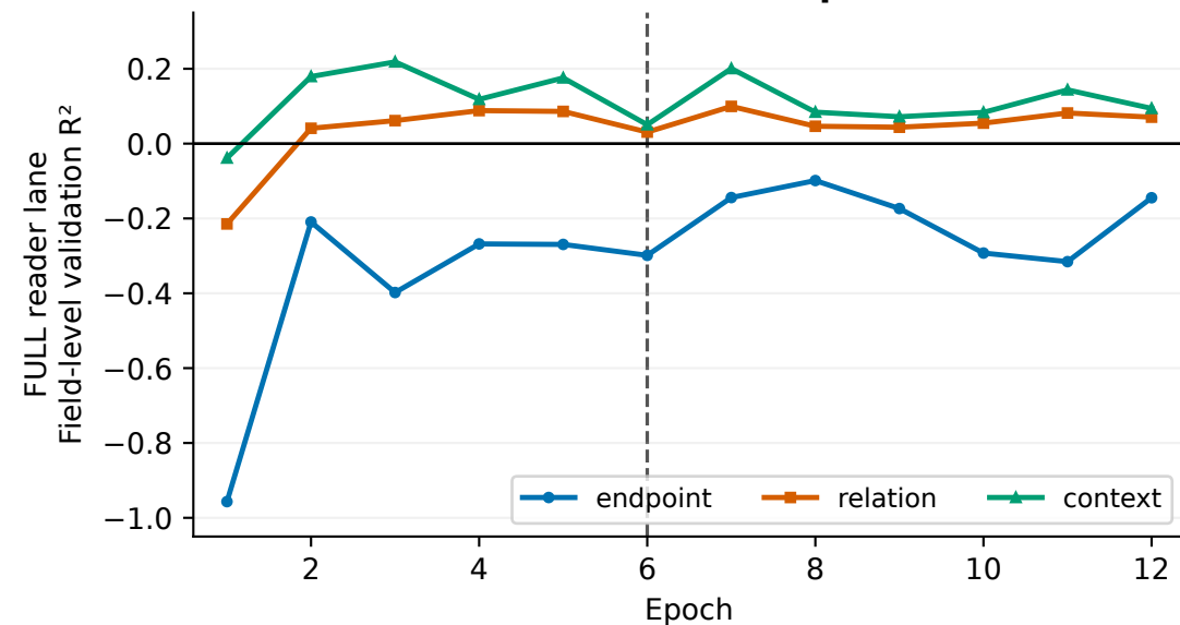
Continuous-coordinate prediction
